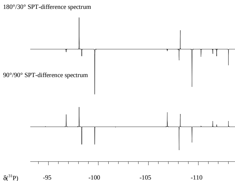
Fig. 5.10: Comparison of the difference spectra from a 180°/30° SPT and a 90°/90° SPT experiment.
