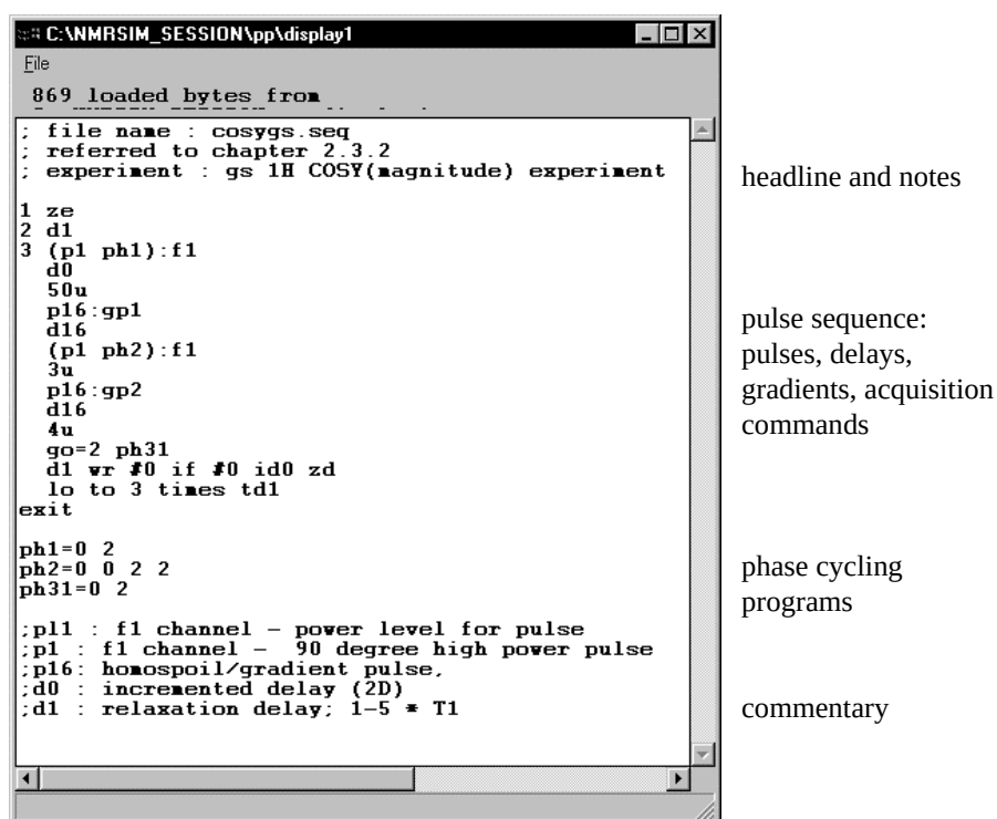
Fig. 4.7: An example of a pulse program: a gradient selected magnitude COSY experiment.
