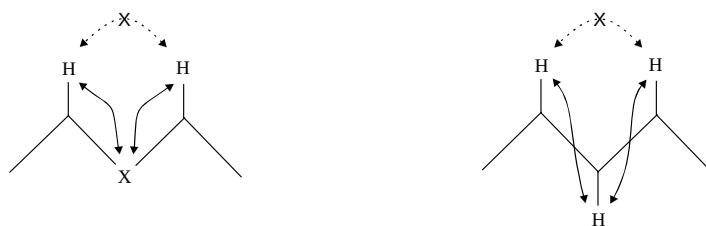
Heteronuclear relay step
