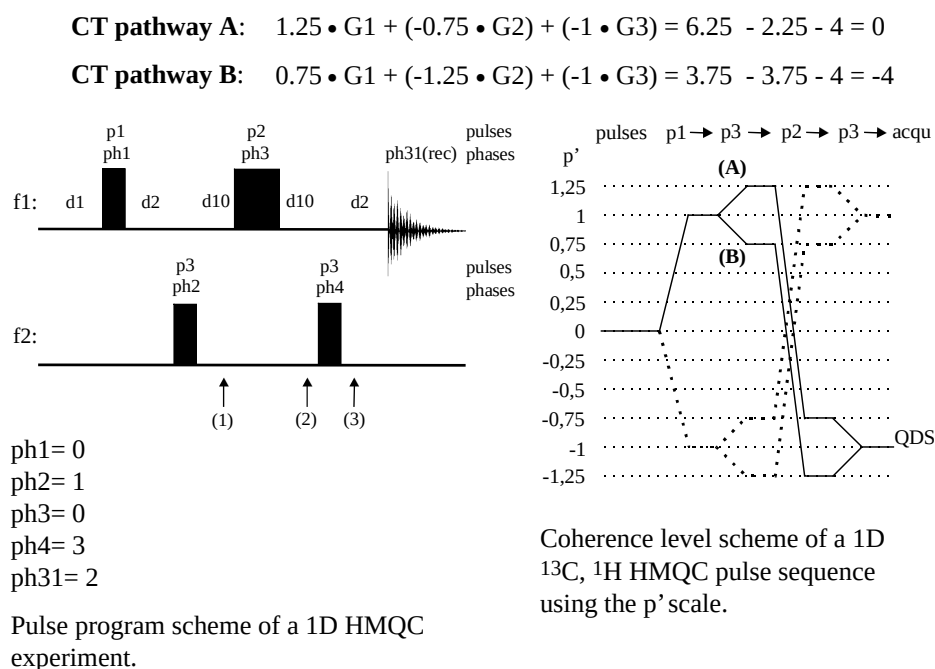
Fig. 2.14: 1D HMQC experiment - Pulse sequence scheme and CT diagram.
