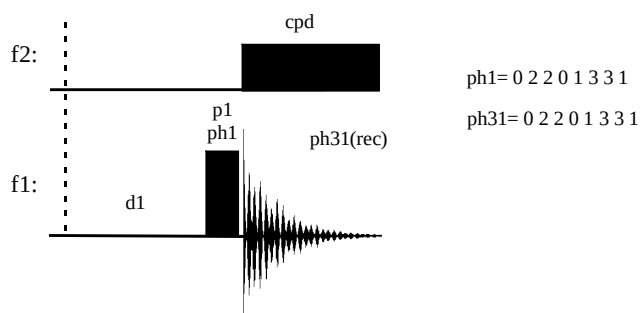
Fig. 4.9: The ^n\text{X}\{^1\text{H}\} experiment. The curly brackets \{^1\text{H}\} denote ^1\text{H} decoupling during data acquisition.
