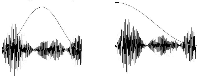
FIDs of the decomposed ^1\text{H} DQ COSY spectrum of Check it 3.3.2.4 , corresponding to rows 71, 235 and 753. Note the applied zero filling.
