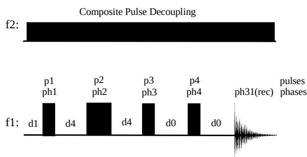
COSY like 2D INADEQUATE experiment.
