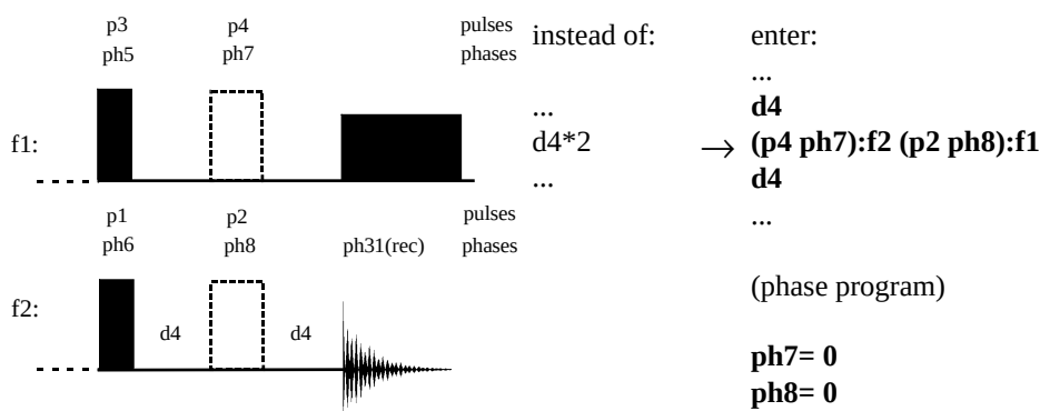
Fig. 5.13: Optional 180^\circ(^{13}\text{C})/180^\circ(^1\text{H}) pulse combination (dotted pulses) to the INEPT-J(H, H)-resolved experiment (left), additional pulse program lines for the pulse combination (right).
