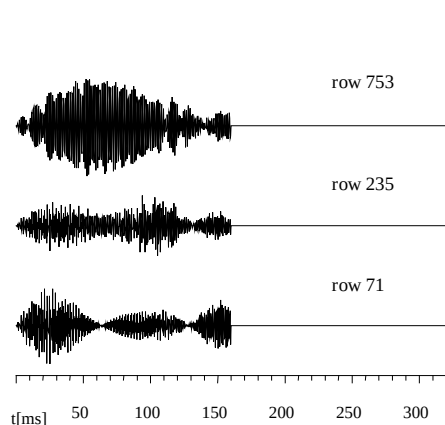
FIDs of the decomposed ^1\text{H} DQ COSY spectrum of Check it 3.3.2.4 , corresponding to rows 71, 235 and 753. Note the applied zero filling.
