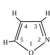
Fig. 5.27: 1,2-oxazole - the test spin system for the INADEQUATE spectra.
