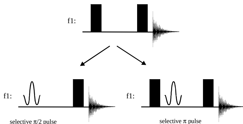
Fig. 5.23: Possible selective pulse schemes to generate a 1D COSY experiment.
