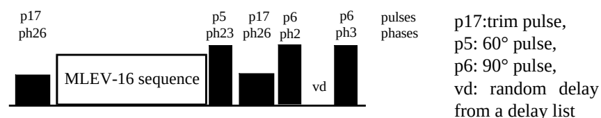
MLEV-17 spinlock sequence with z-filter and trim pulses.
