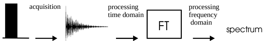
Fig. 3.2: Flow chart - acquisition and processing.
